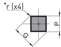
PB-RFEV Square
