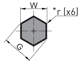
P_-PPEH Hexagon
