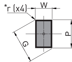
P_-PPER Rectangle
