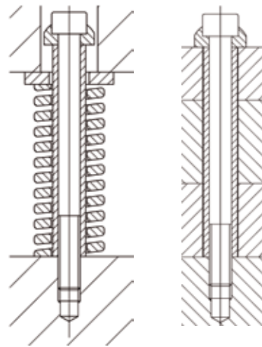
Assembly examples
