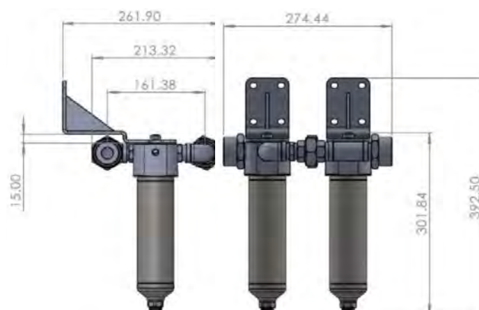
Expel 60M 6001-012 - Acier inoxydable
